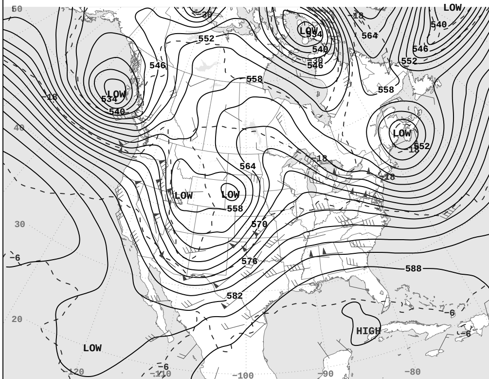
MON, MAY 19, 2025 500-Millibar Height Contours at 7:00 A.M. E.S.T.
