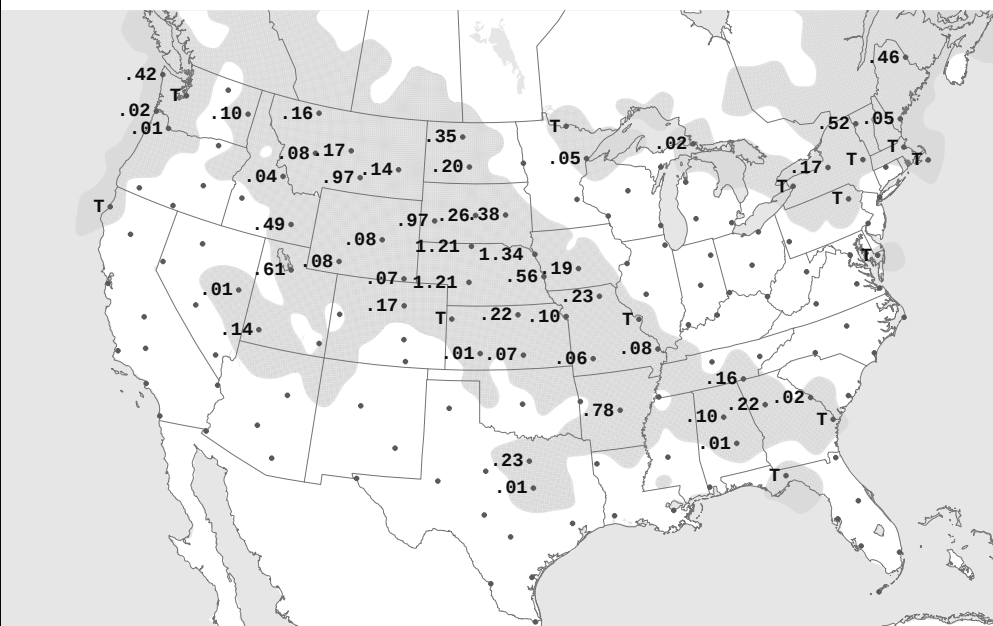
MON, MAY 19, 2025 24-hour Precipitation Areas and Amounts Ending 7:00 A.M. E.S.T.
