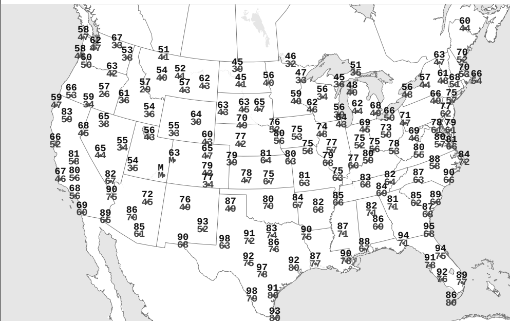
MON, MAY 19, 2025 Highest and Lowest Temperature
